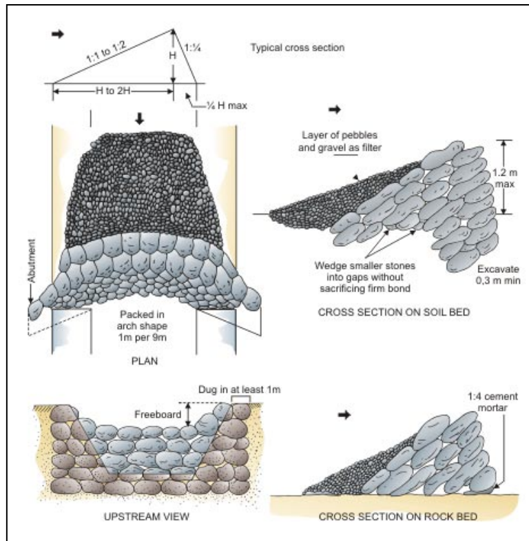
Figure 2. Stone packed structure.
